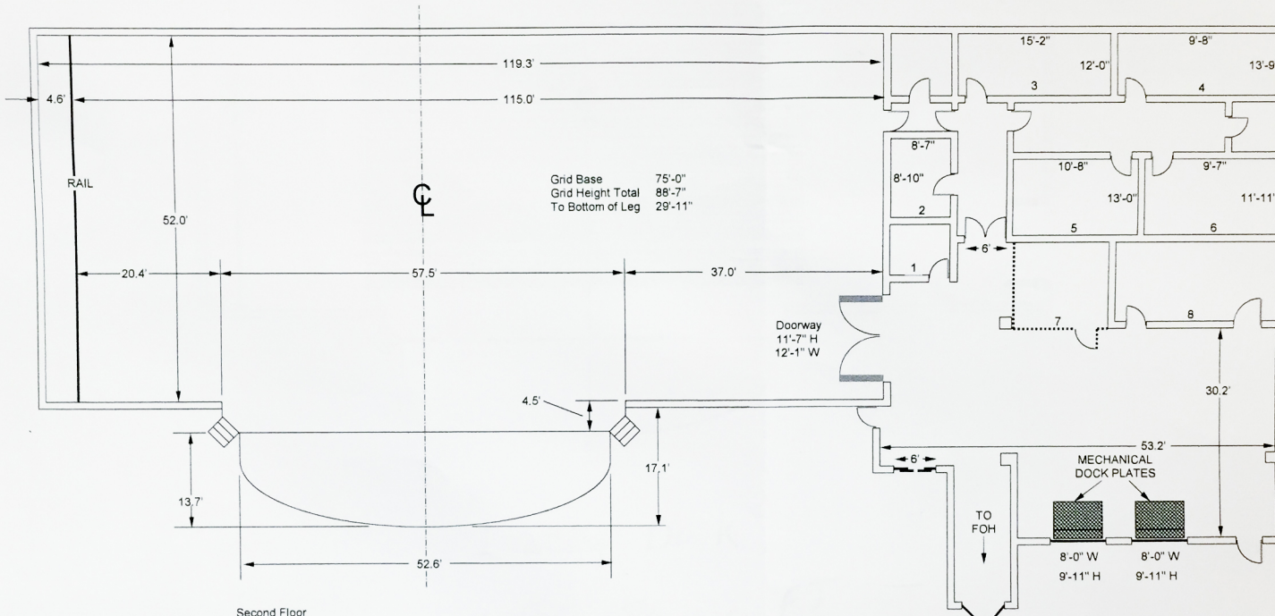
Second Floor
